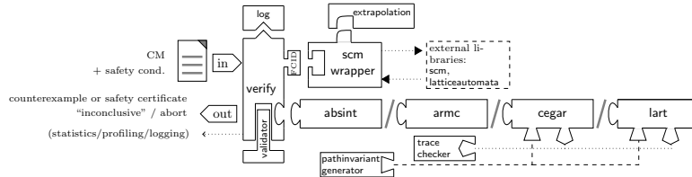
Fig. 1. Modular Architecture of McScM’s Verification Tools
